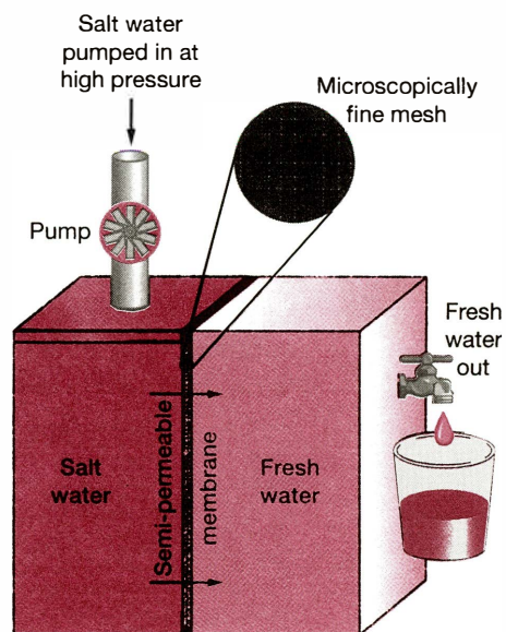
Reverse osmosis
